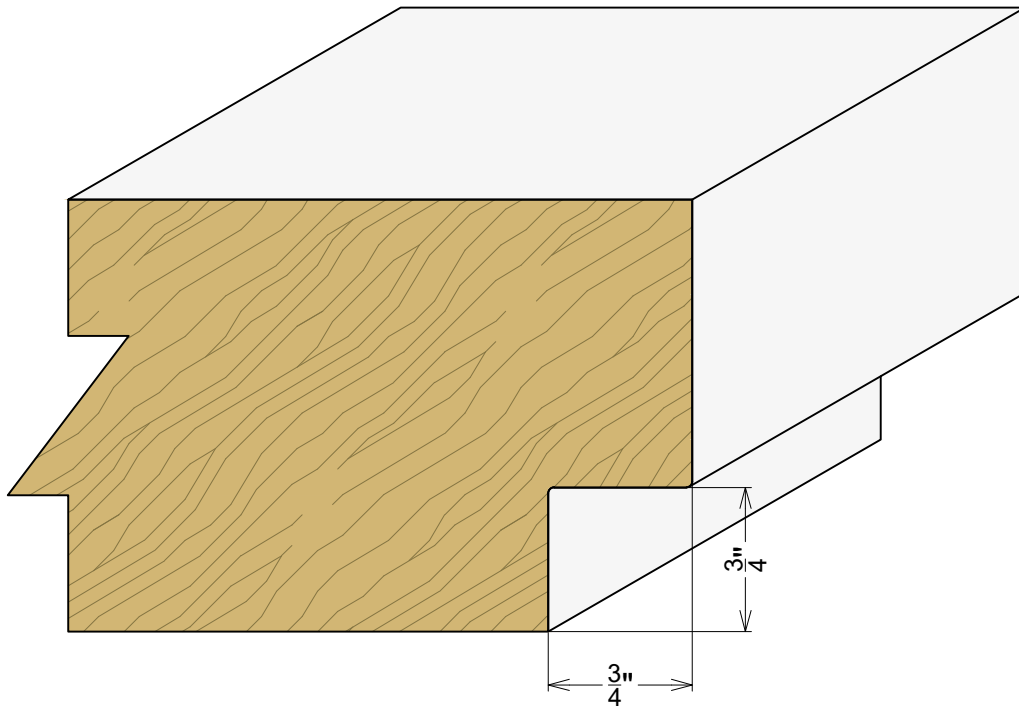
AP 9085 2-1/4" Door Profile
