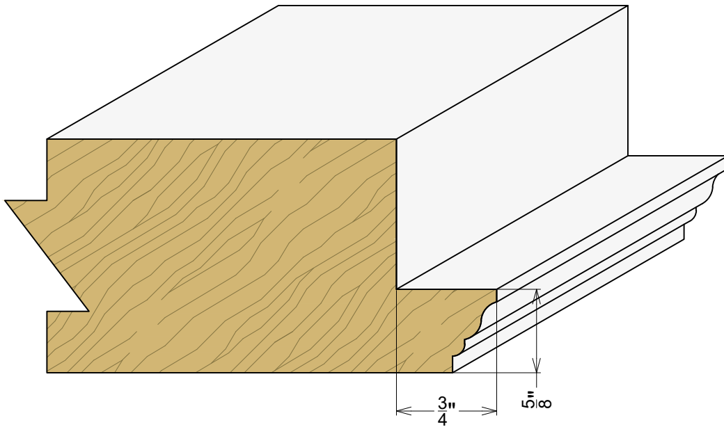
AP 9091 1-3/4" Door Profile
