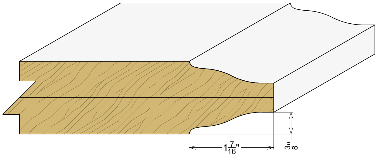
AP 9101 1-1/4" Panel Profile
