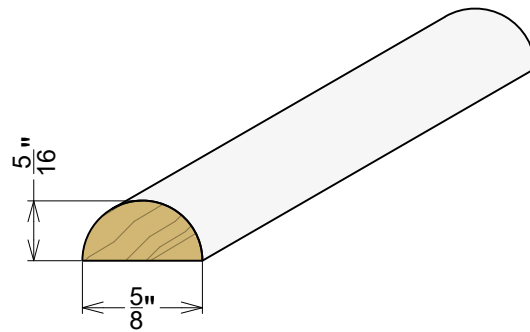
Half Round 5/8" Dia.
