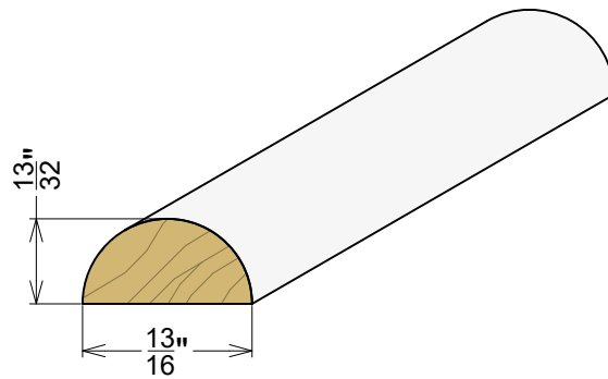
Half Round 13/16" Dia.
