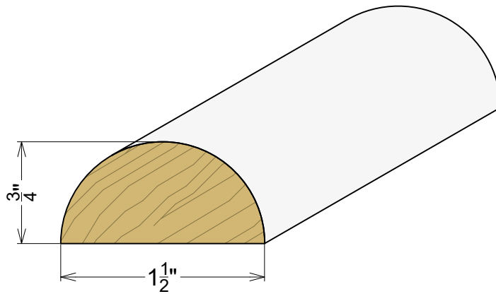
Half Round 1-1/2" Dia.
