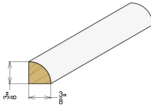
Cove 3/8" Radius
