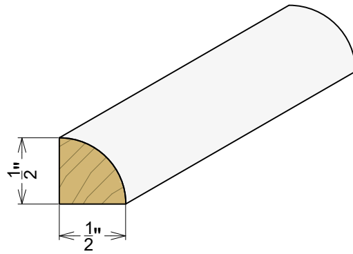
Cove 1/2" Radius
