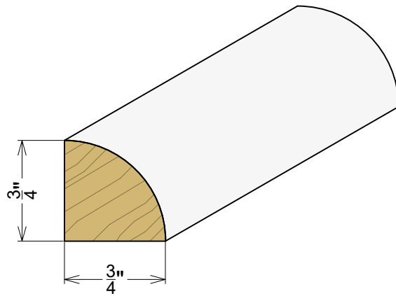
Cove 3/4" Radius
