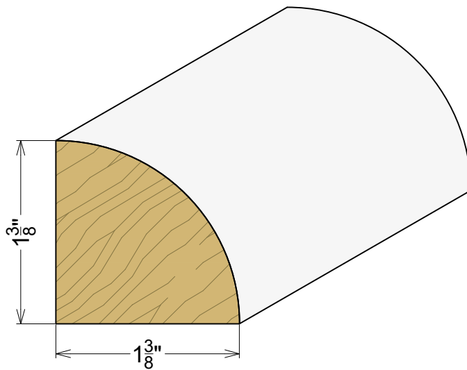
Cove 1-3/8" Radius
