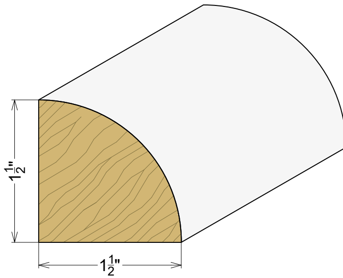
Cove 1-1/2" Radius
